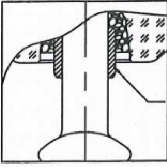
锌套 Sacrificial sleeve > 99.8% Zinc
